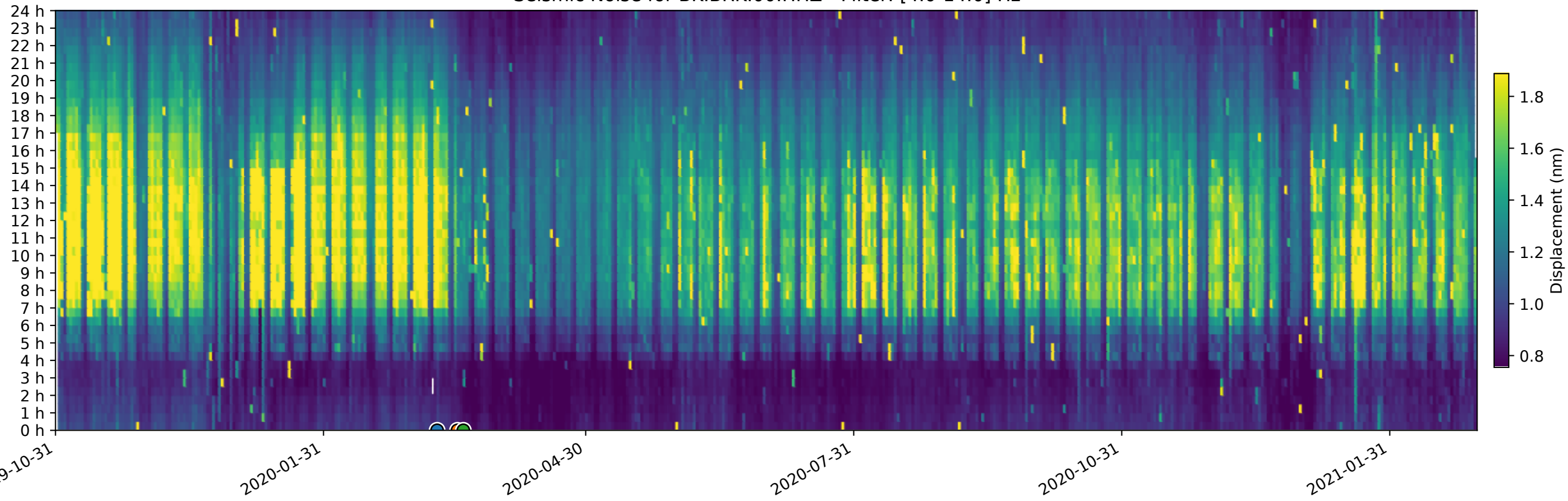
Seismic Noise for BK.BRK.00.HHZ - Filter: [4.0-14.0] Hz
