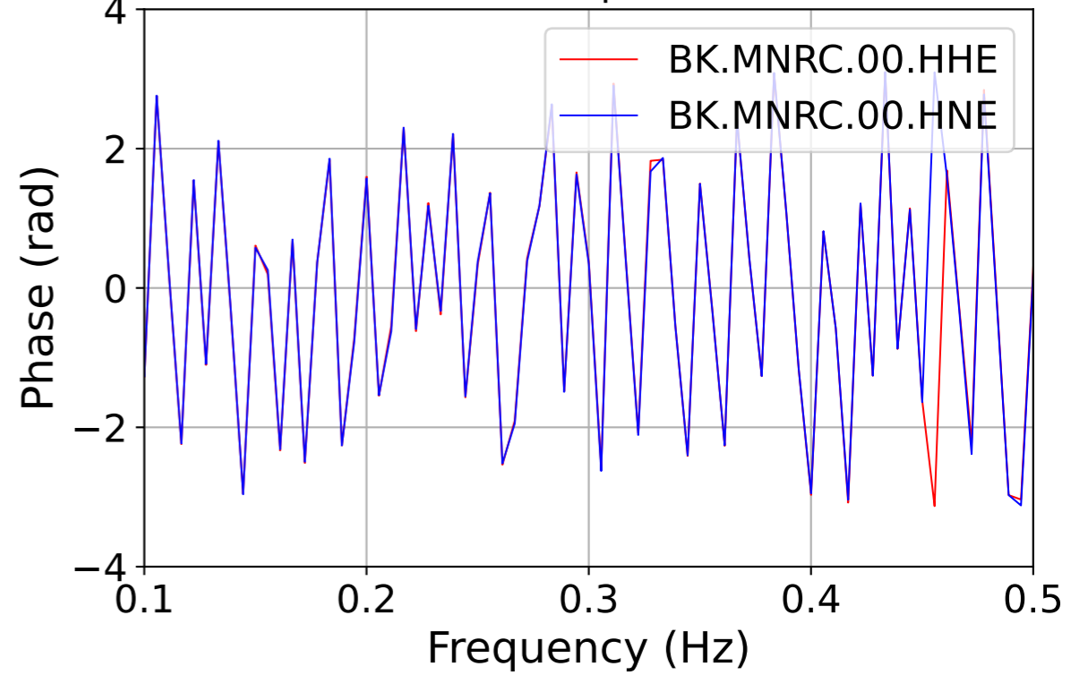
Phase spectra
