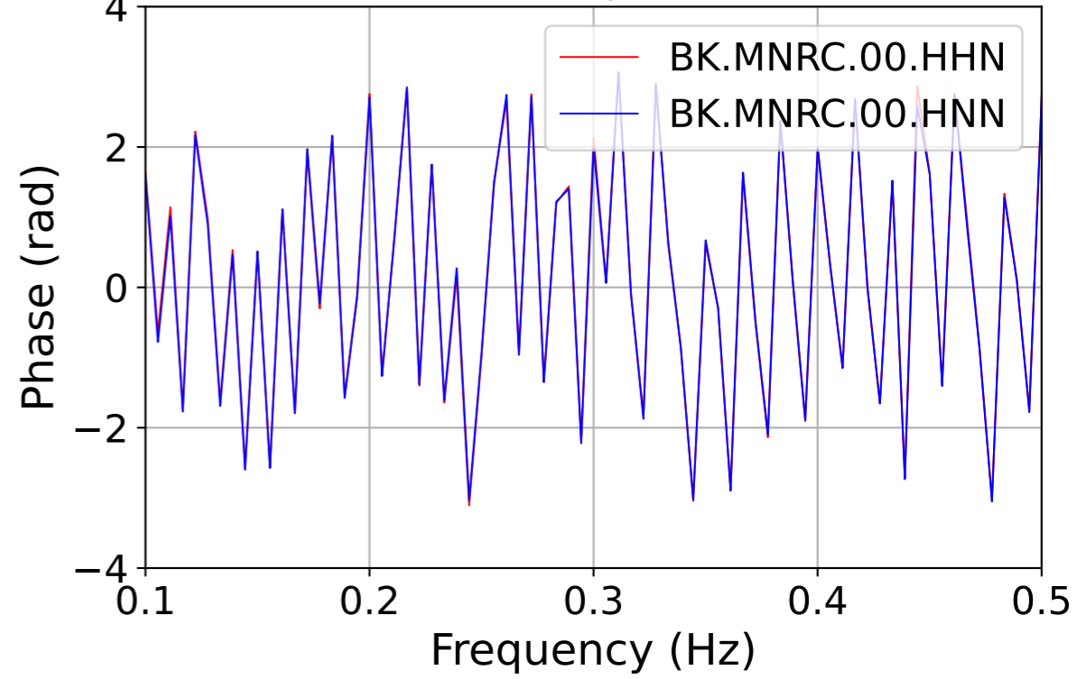
Phase spectra
