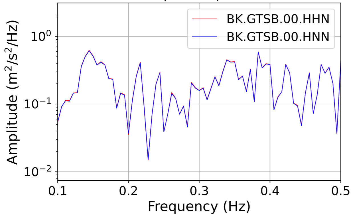
Amplitude spectra
