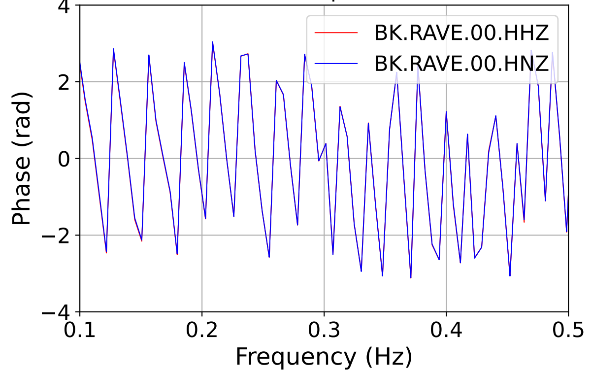
Phase spectra
