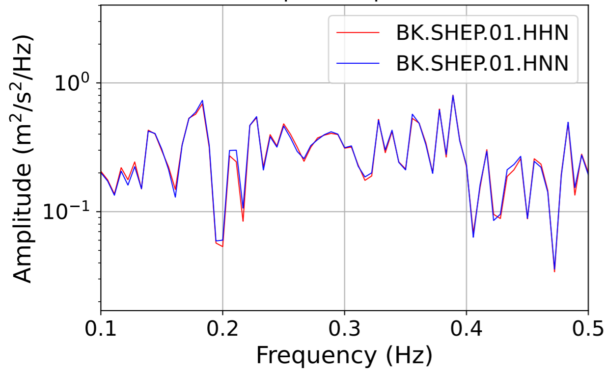
Amplitude spectra
