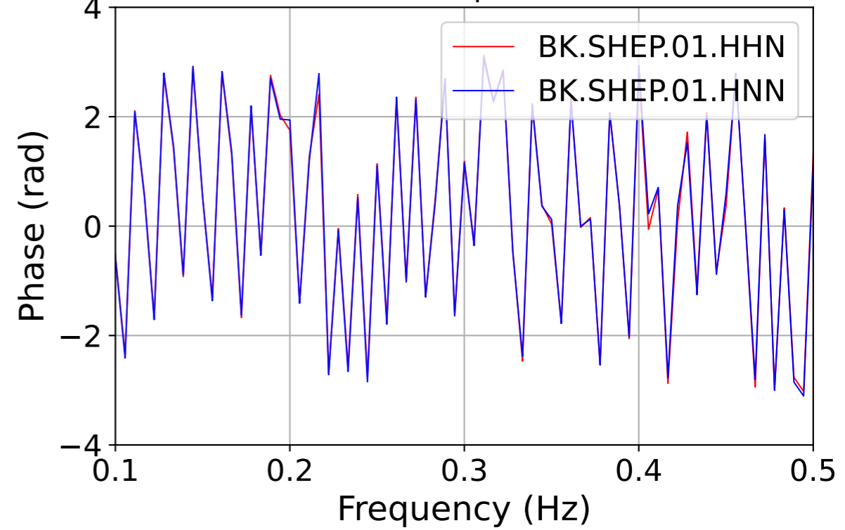
Phase spectra
