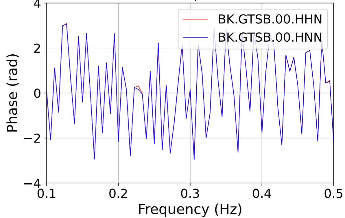
Phase spectra
