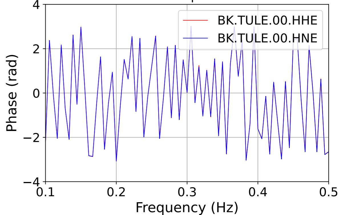
Phase spectra
