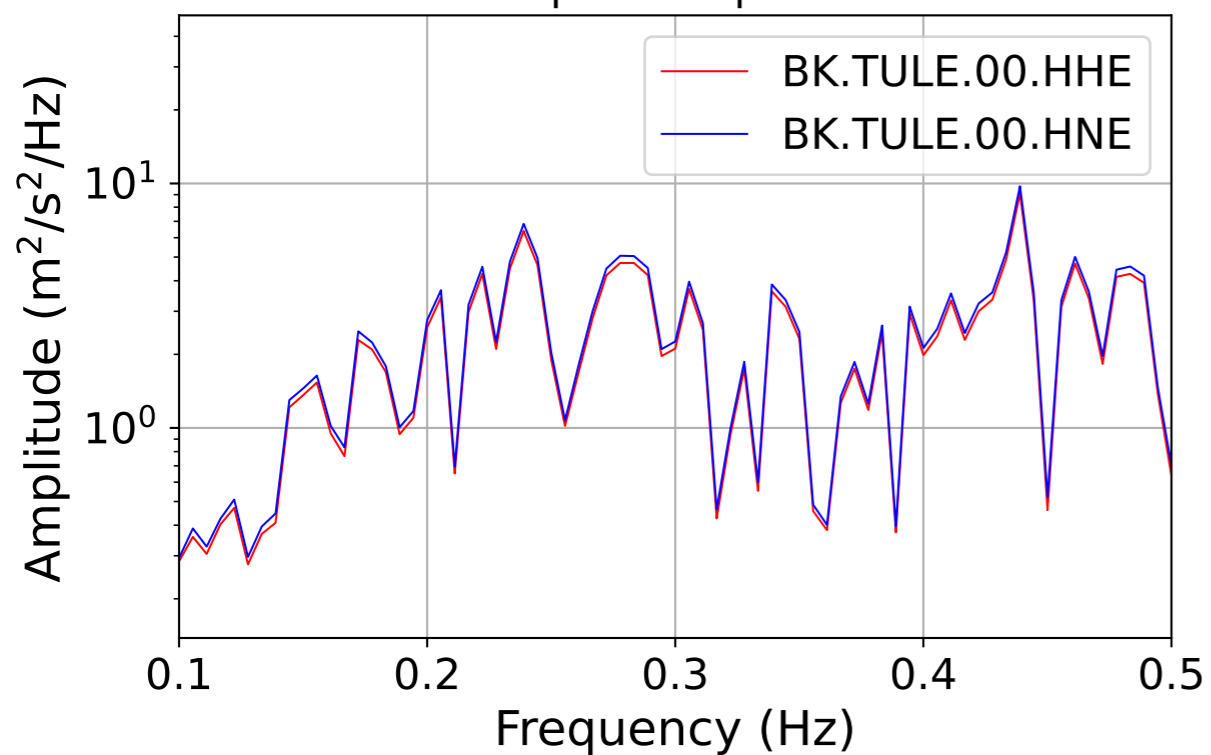
Amplitude spectra
