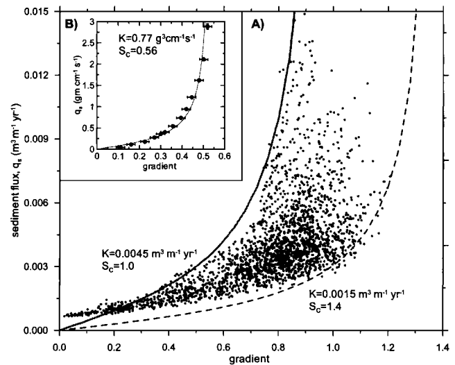
Figure 8. A. Plot of sediment flux versus local hillslope gradient derived from high resolution topographic data in the Oregon Coast Range [from Roering et al., 1999]. Parameters reported are best-fit estimates of equation 10 in the text. B. Measured sediment flux versus gradient derived from acoustically-disturbed sandbox experiments [Roering et al., 2001]. Line passing through data is for the best fit values of equation 10.
