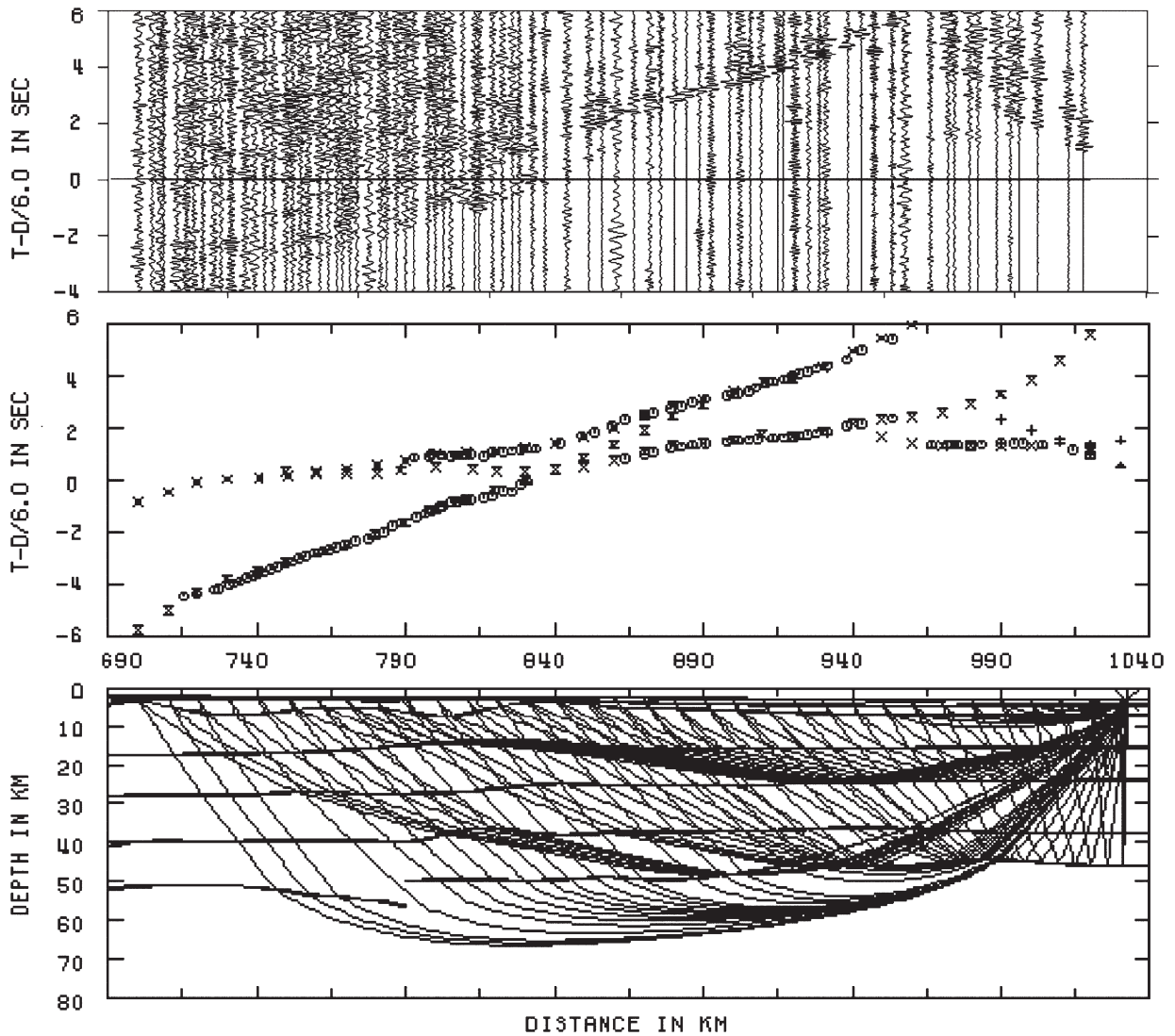
Fig. 3. Record section of Profile 973 from Shot Point 1032 (upper), its ray-tracing diagram (bottom) and travel-time curves (middle). The ray-tracing diagram is of Pg, PMP and Pn waves for the final 2-D model. The lower part shows the comparison between observed and calculated travel-times. Circles represent calculated travel-times, while signs “+” and “x” represent observed data.
