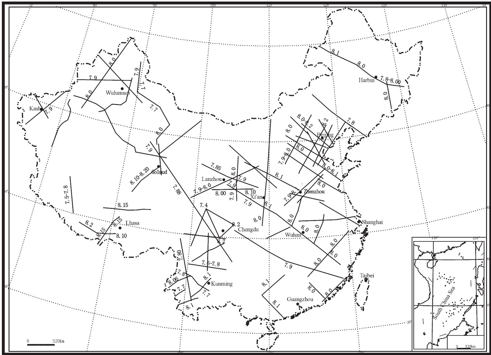
Fig. 6. Seismic velocities of the uppermost mantle from Pn waves. Pn velocities are generally lower in eastern China as compared with those of the Tibetan Plateau.
