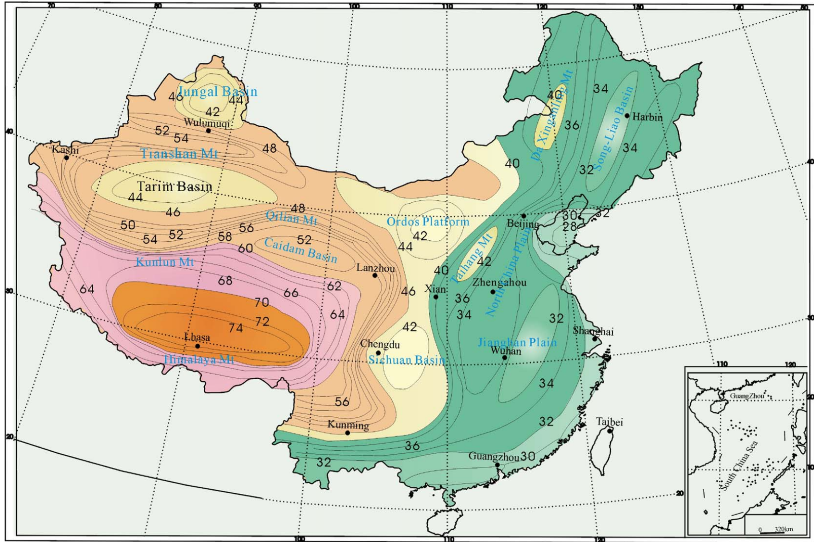
Fig. 4. Contour map of crustal thickness obtained from DSS data (Fig. 1). Contour interval is 2 km. Crustal thickness ranges from 28 to 46 km in eastern China, and from 42 to 74 in western China. The margins of the Tibetan plateau are marked by a steep gradient in crustal thickness.
