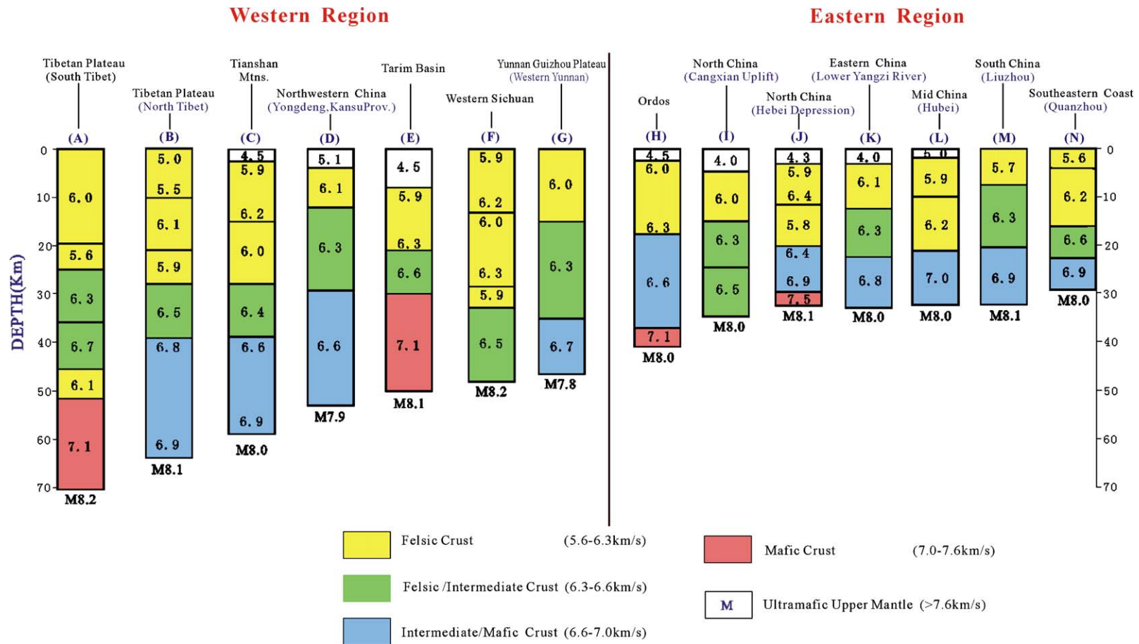
Fig. 5. Representative seismic velocity–depth functions for fourteen regions of China that can be divided into a western region (A–G) and an eastern region (H–N). Letters A–N indicate the position of each column as shown in Fig. 2. Note the low-velocity layer beneath the Tibetan Plateau, Western Sichuan, and Tianshan Mountains that extends to ~25 km depth in the western region. The high-velocity basal crustal layer ( \geq 7.1 km/s) referred to in the text is indicated in red.
