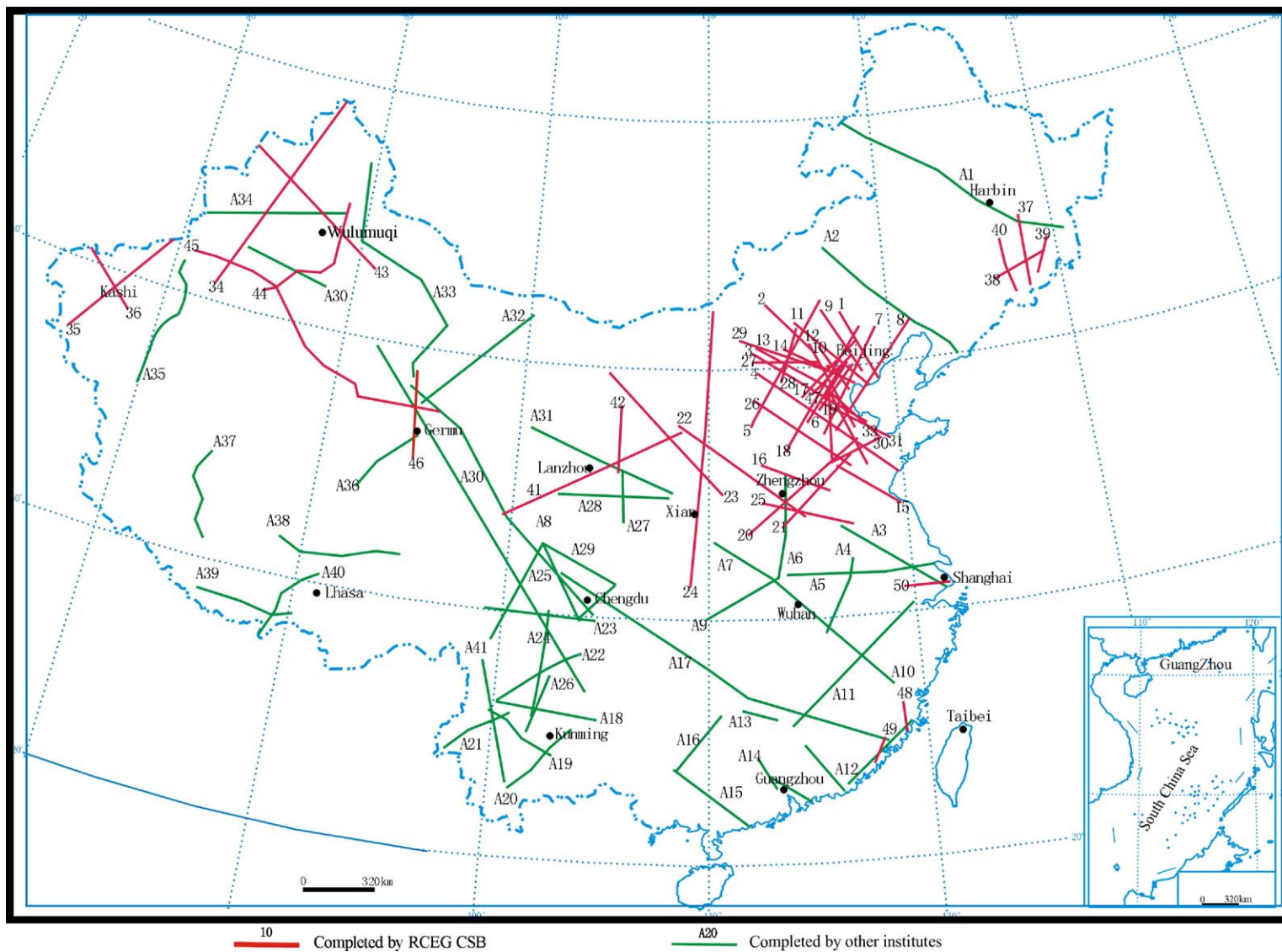
Fig. 1. Position map of refraction/wide angle reflection profiles in mainland China. Red lines represent profiles completed by RCEG, CEA (Research Center of Exploration Geophysics, China Earthquake Administration). The number of each profile is written near it and is the same as that listed in Table 1. Green lines are profiles by other institutes. Their profile numbers are represented by a capital letter “A” and a number and are the same as those listed in Table 2.
