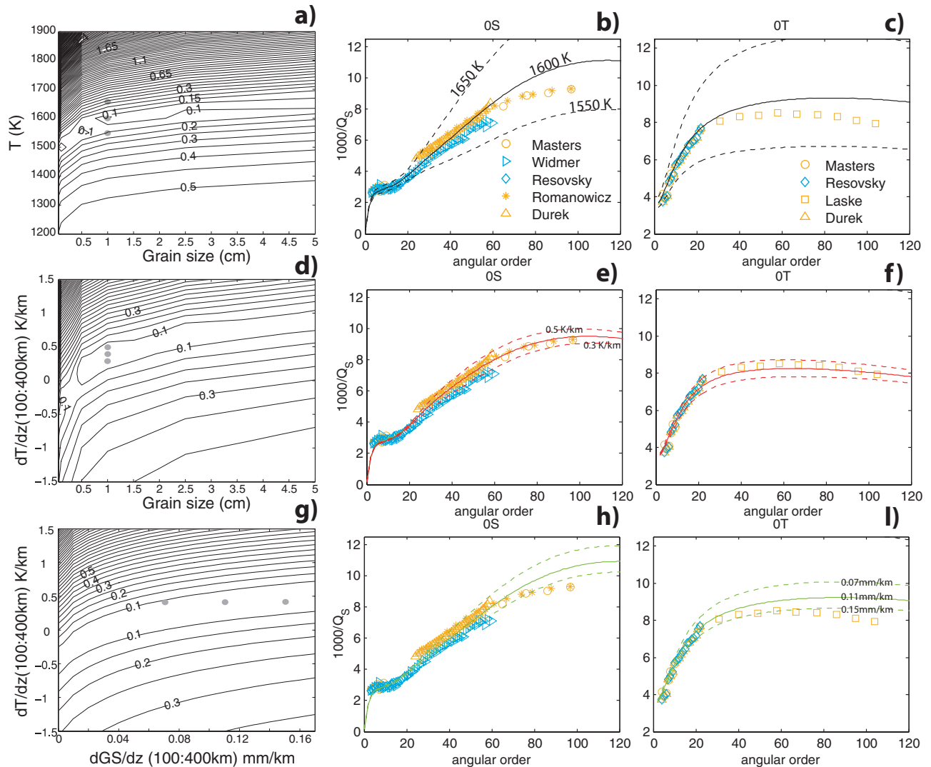
Figure 3. Misfit values for isotherms at constant grain sizes (top panel), for linear thermal gradients between 100 and 400 km, starting from a T_{\text{REF}} = 1550 K (middle panel), and for the same thermal structure but allowing grain size to linearly increase from 100 to 400 km starting from a GS_{\text{REF}} = 1 mm. Measurements for top and middle panel have been performed at grain sizes of 0.05, 0.1, 0.5, 1, 2.5 and 5 cm every 50 K (top panel) and every 0.1 \text{ K km}^{-1} (middle and bottom panel). Data for grain-size gradients in bottom panel are every 0.01 \text{ mm km}^{-1} . Panels on the right-hand side show computed predictions for {}_0S and {}_0T compared with the observations for models represented by grey circles on the left-hand panels. Predictions for overtones are given in the supporting information (Appendix S1). The P - T and GS -dependent model is Faul & Jackson (2005). Reference period is 150 s. V^* is \sim 12 \times 10^{-6} \text{ m}^3 \text{ mol}^{-1} . Background elastic model is iPREF (see text).
