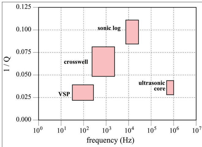
Figure 2. Intrinsic P-wave attenuation 1/Q as determined by Sams et al. (1997) on rocks from the same geologic sequence. The number of Q estimates coming from different depth ranges that fall within each rectangle above are: 40 VSP, 69 crosswell, 854 sonic log, and 46 ultrasonic core measurements.
