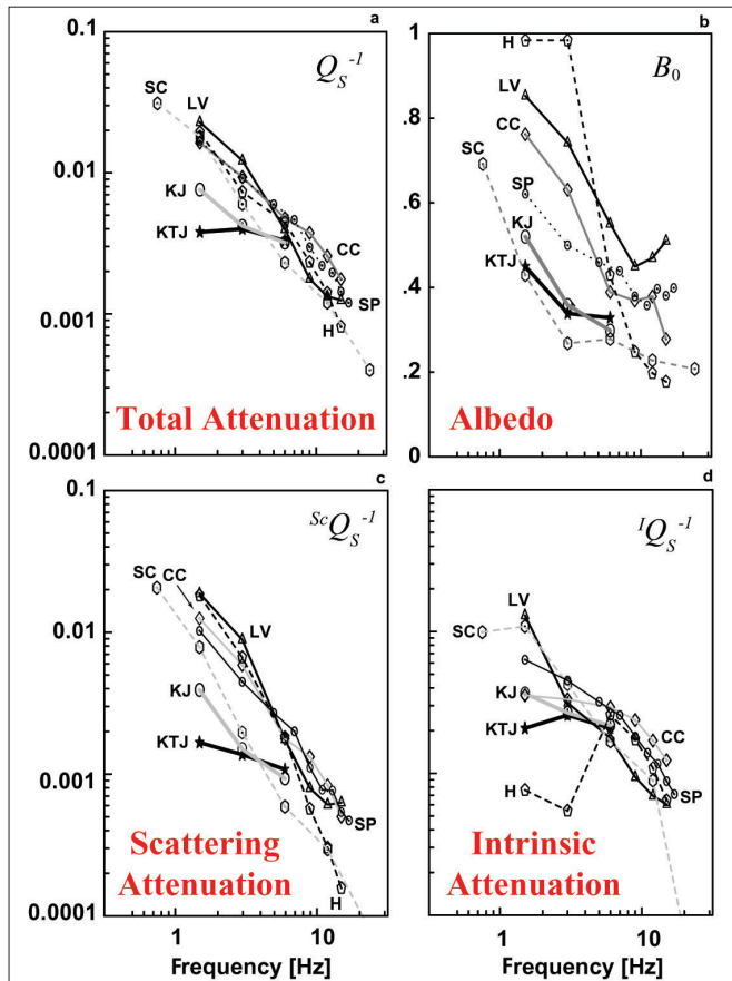
Figure 3. S-wave attenuation determined from regional seismic data collected around the world (Sato and Fehler, 1998). The attenuation so determined corresponds to the average attenuation in each of the various crustal regions. The albedo is defined as B_0 = Q_{sc}^{-1}/Q_{total}^{-1} . The various curves in each graph represent data from: KTJ=Kanto-Tokai, Japan; KJ=Kanto, Japan; LV=Long Valley, California; H=Hawaii; SC=Southern California; SP=Southern Spain; and CC=Central California.
