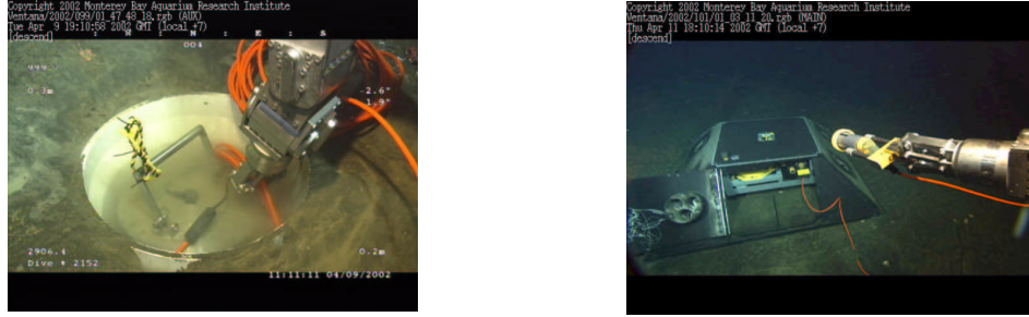
Figure 2: left: Installation of the seismometer package inside the PVC caisson. This was later completely covered by glass beads. Right: Trawl-resistant enclosure for the recording and battery packages. This snapshot was taken as the ROV Ventana was bringing the cable from the seismometer package in order to connect it onto the recording package. The first time such a remote underwater connection was attempted during the MOISE experiment, it took 2.5 hours to succeed and led to a redesign of the geometry of the instrument packages. The ROV operators are now able to do this routinely in less than 5-10mn.
