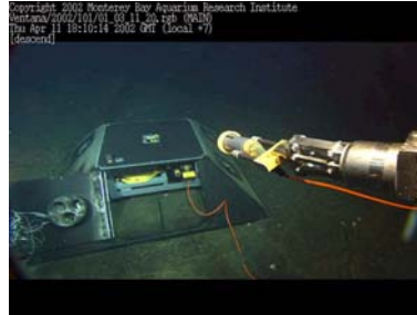
Figure 2: left: Installation of the seismometer package inside the PVC caisson. This was later completely covered by glass beads. Right: Trawl-resistant enclosure for the recording and battery packages. This snapshot was taken as the ROV Ventana was bringing the cable from the seismometer package in order to connect it onto the recording package. The first time such a remote underwater connection was attempted during the MOISE experiment, it took 2.5 hours to succeed and led to a redesign of the geometry of the instrument packages. The ROV operators are now able to do this routinely in less than 5-10mn.
